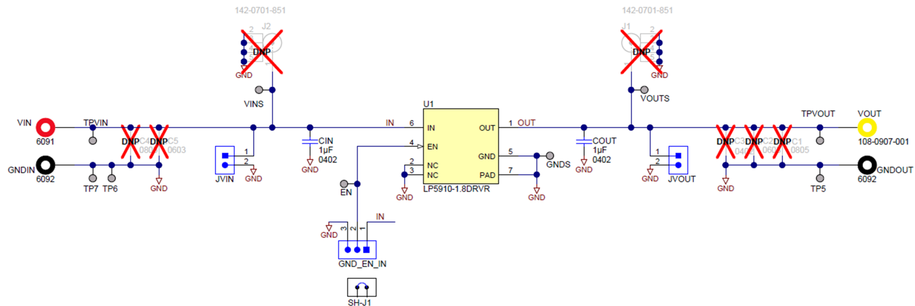
Figure 10. LP5910DRVEVM Schematic
