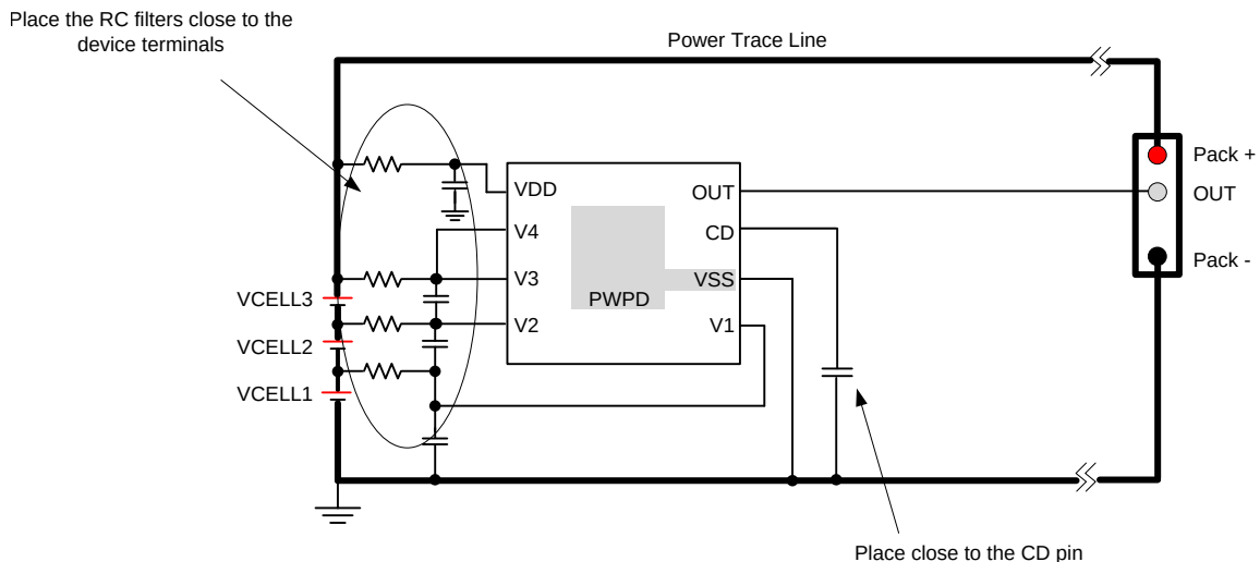
Figure 17. Layout
