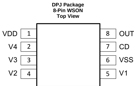
Pin Functions
