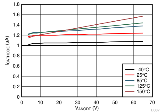
Figure 2. Operating Quiescent Current vs Supply Voltage
