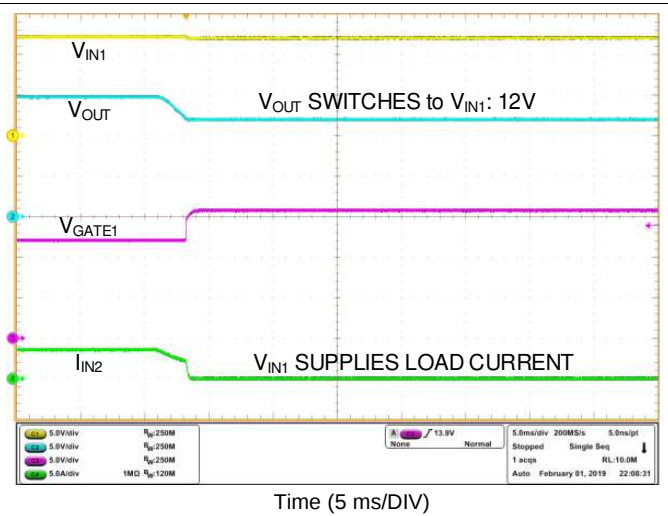
Figure 33. ORing V_{IN2} to V_{IN1} Switch Over
