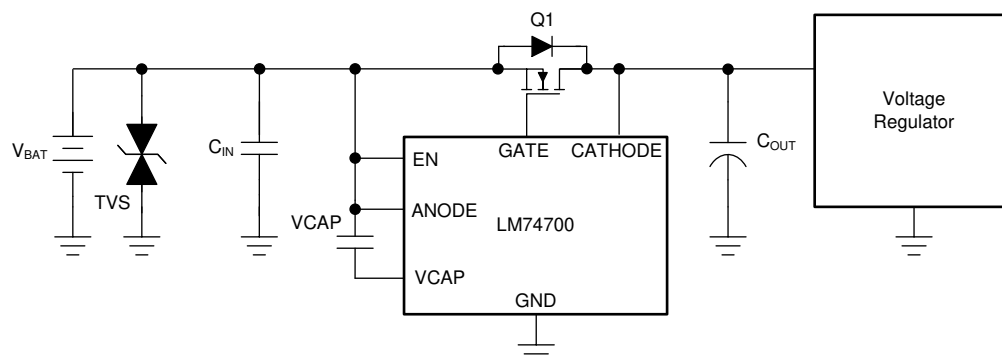
Figure 19. Typical Application Circuit
