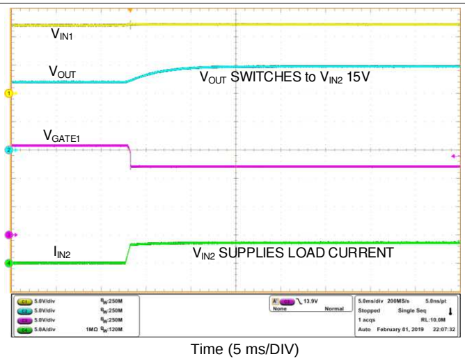
Figure 31. ORing V_{IN1} to V_{IN2} Switch Over
