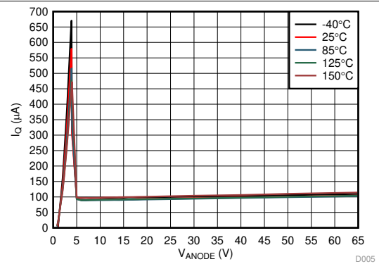
Figure 2. Operating Quiescent Current vs Supply Voltage
