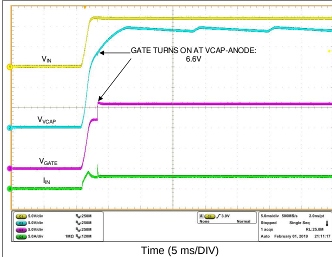
Figure 26. VCAP during startup at 3-A Load
