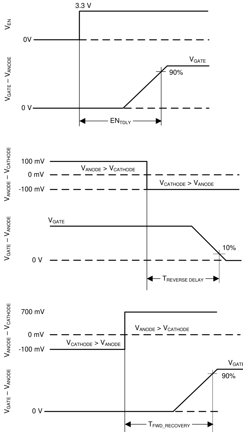
Figure 16. Timing Waveforms
