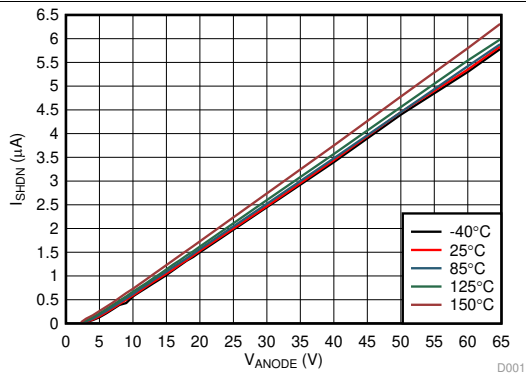
Figure 1. Shutdown Supply Current vs Supply Voltage
