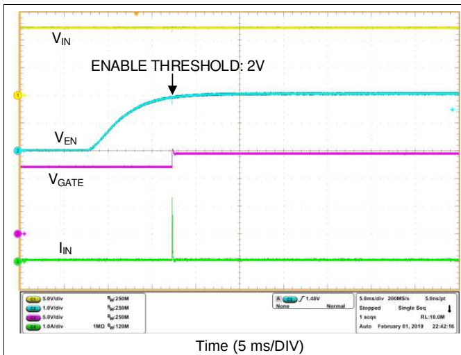
Figure 28. Enable Threshold
