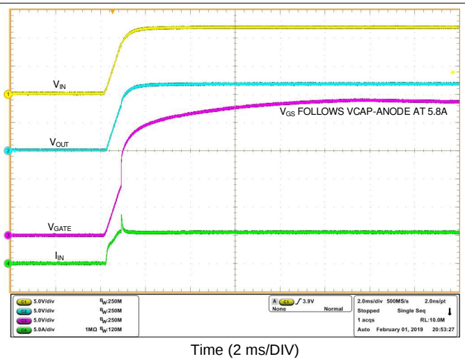
Figure 25. Startup with 5.8-A Load
