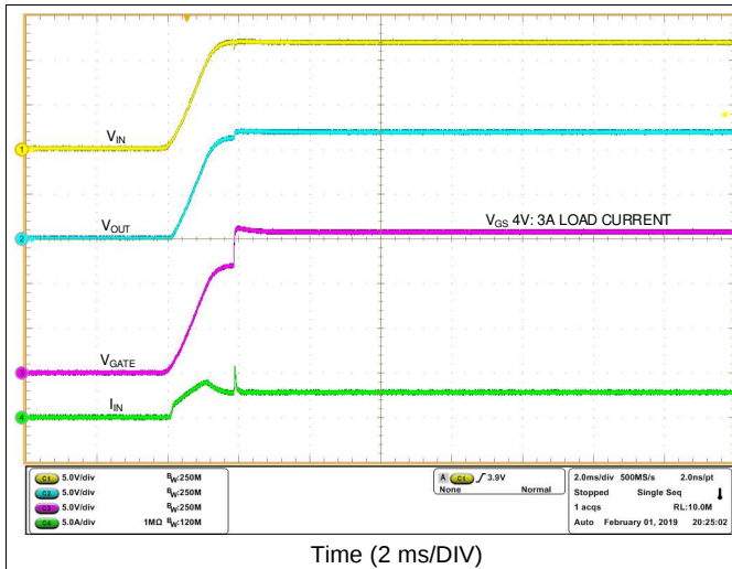
Figure 24. Startup with 3-A Load
