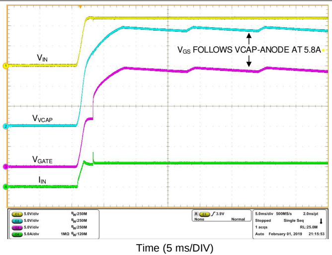
Figure 27. VCAP during startup at 5.8-A Load
