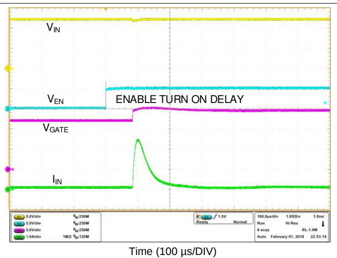
Figure 29. Enable Turn ON Delay
