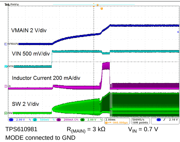
Figure 78. Startup
