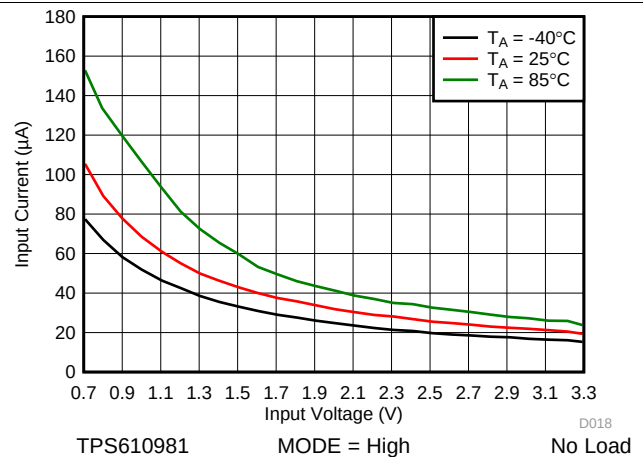
Figure 44. Input Current vs Input Voltage (Active Mode)
