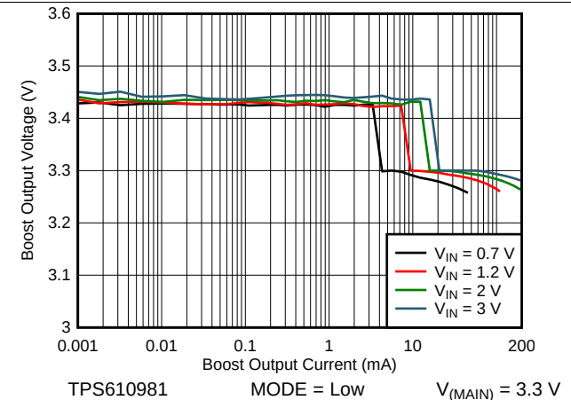
Figure 30. Boost Load Regulation (Low Power Mode)
