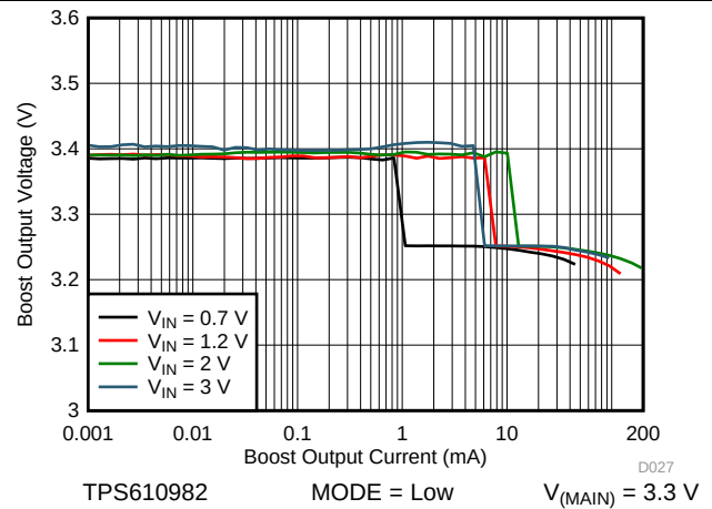
Figure 32. Boost Load Regulation (Low Power Mode)
