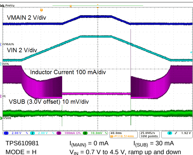
Figure 76. Line Regulation
