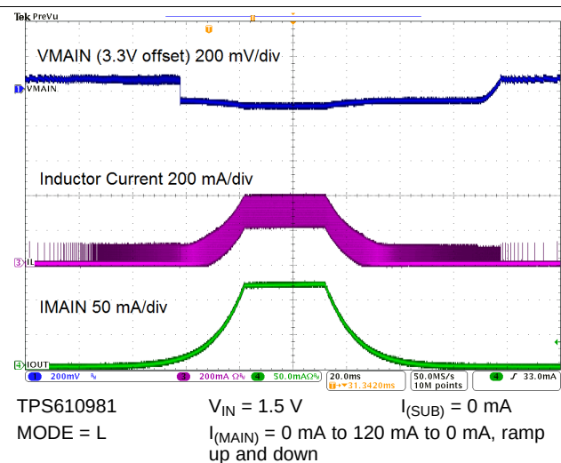
Figure 74. Load Regulation
