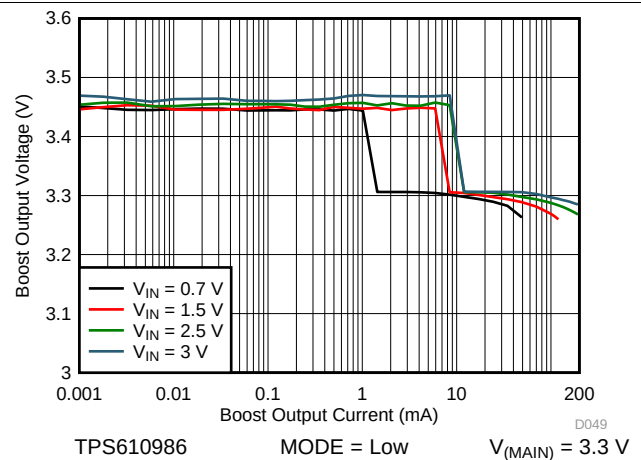
Figure 36. Boost Load Regulation (Low Power Mode)
