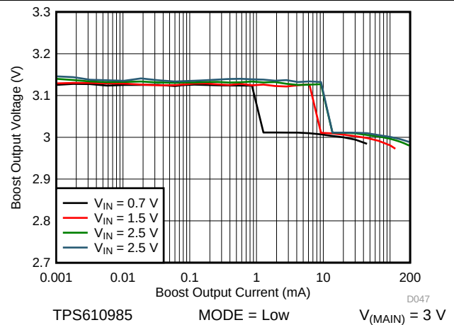
Figure 34. Boost Load Regulation (Low Power Mode)
