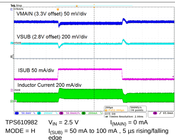
Figure 91. LDO Load Transient Response
