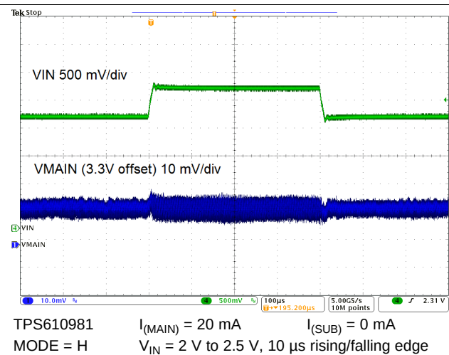
Figure 72. Line Transient Response
