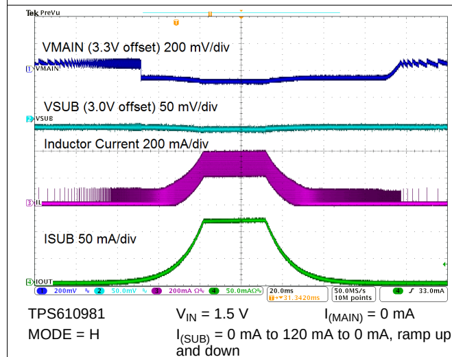
Figure 75. Load Regulation
