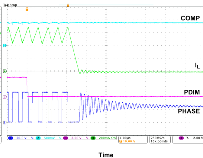
Figure 18. PDIM Falling
