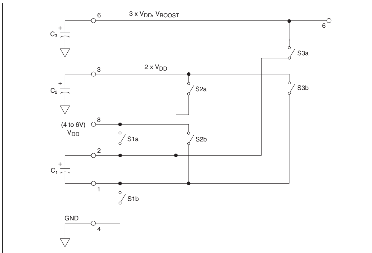
FIGURE 3-3: Voltage Booster.
