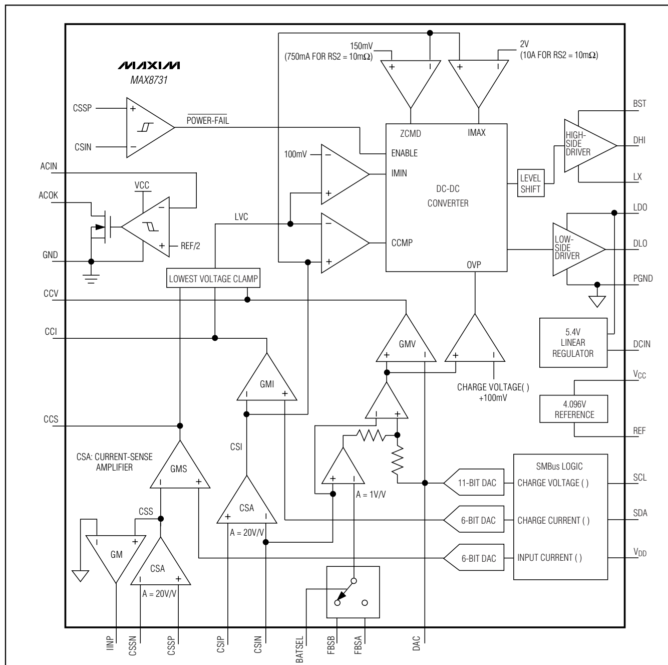
Figure 2. Functional Diagram
