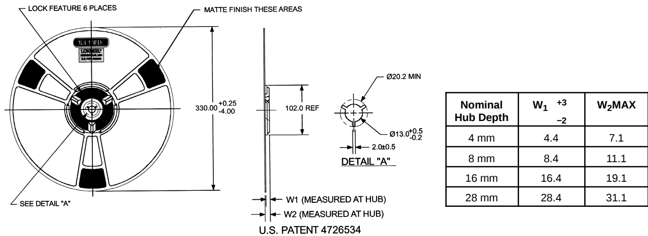
Figure 15. Reel Dimensions
