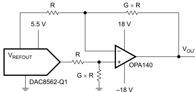
Figure 99. Bipolar Output Range Circuit Using DAC8562-Q1
