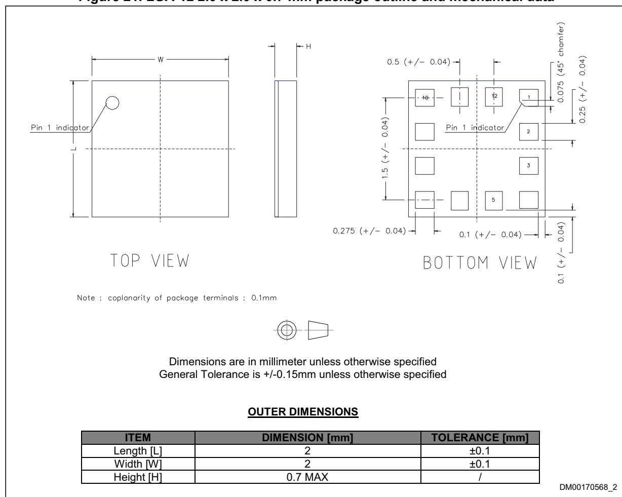
Figure 21. LGA-12 2.0 x 2.0 x 0.7 mm package outline and mechanical data
