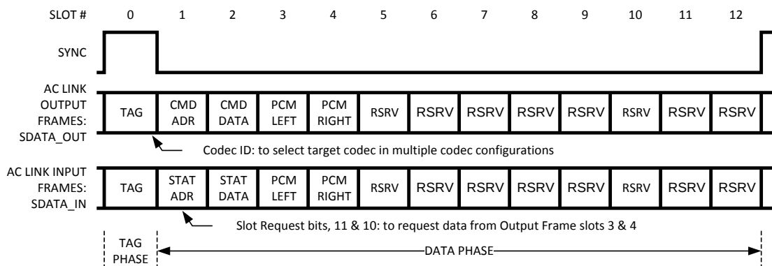
Figure 15. AC Link Bidirectional Audio Frame
