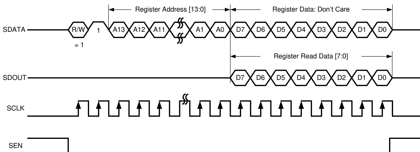
Figure 145. Serial Register Read Timing Diagram
