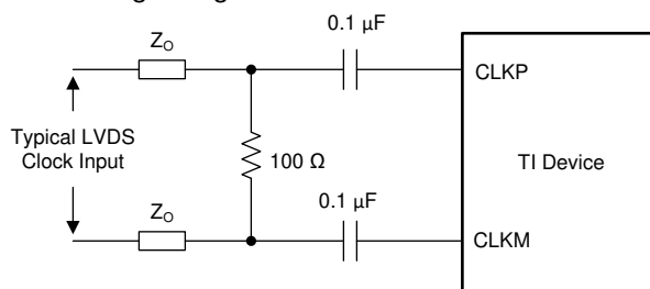
Figure 133. LVDS Clock Driving Circuit
