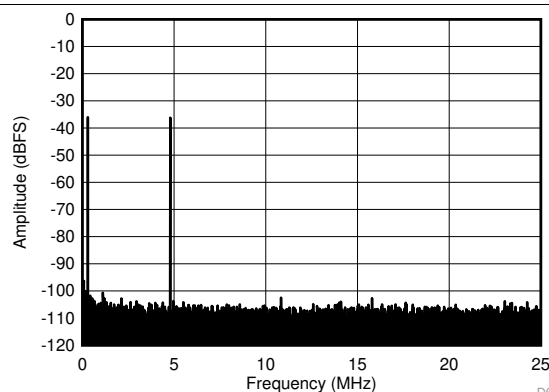
Figure 40. FFT for 450-MHz Input Signal (Dither Off)
