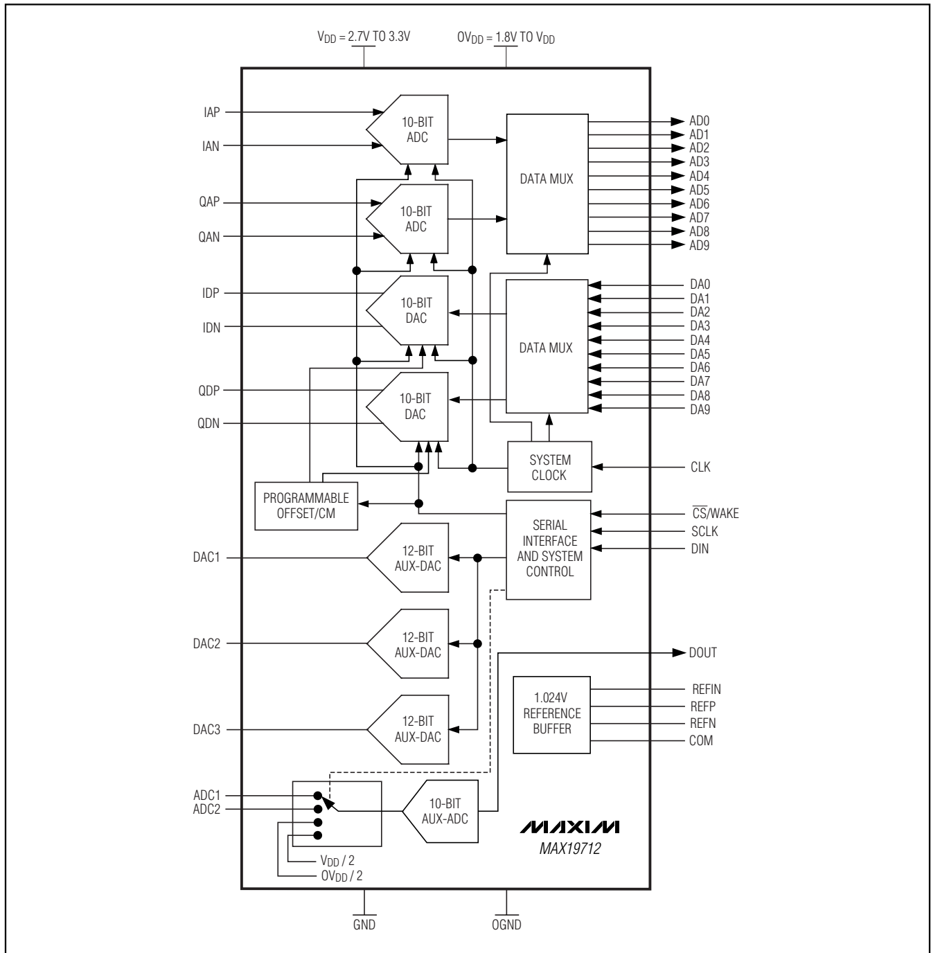
Functional Diagram
