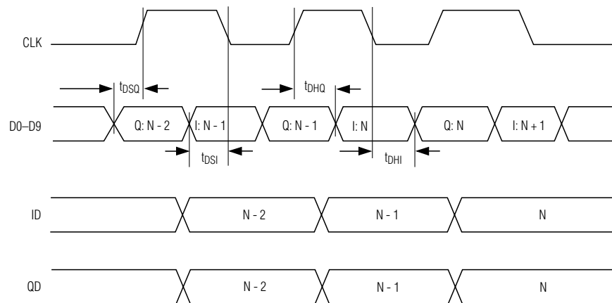
Figure 5. Tx DAC System Timing Diagram
