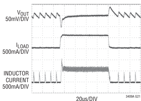
Load Step 50mA to 600mA, Burst Mode Operation, V_{IN} = 3.6\text{V} , V_{OUT} = 1.8\text{V}
