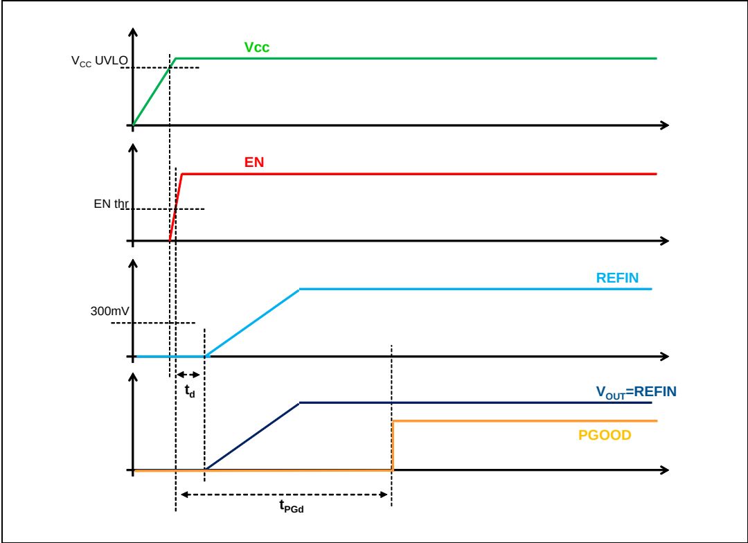
Figure 5. PM8908 turn-on (tracking startup)
