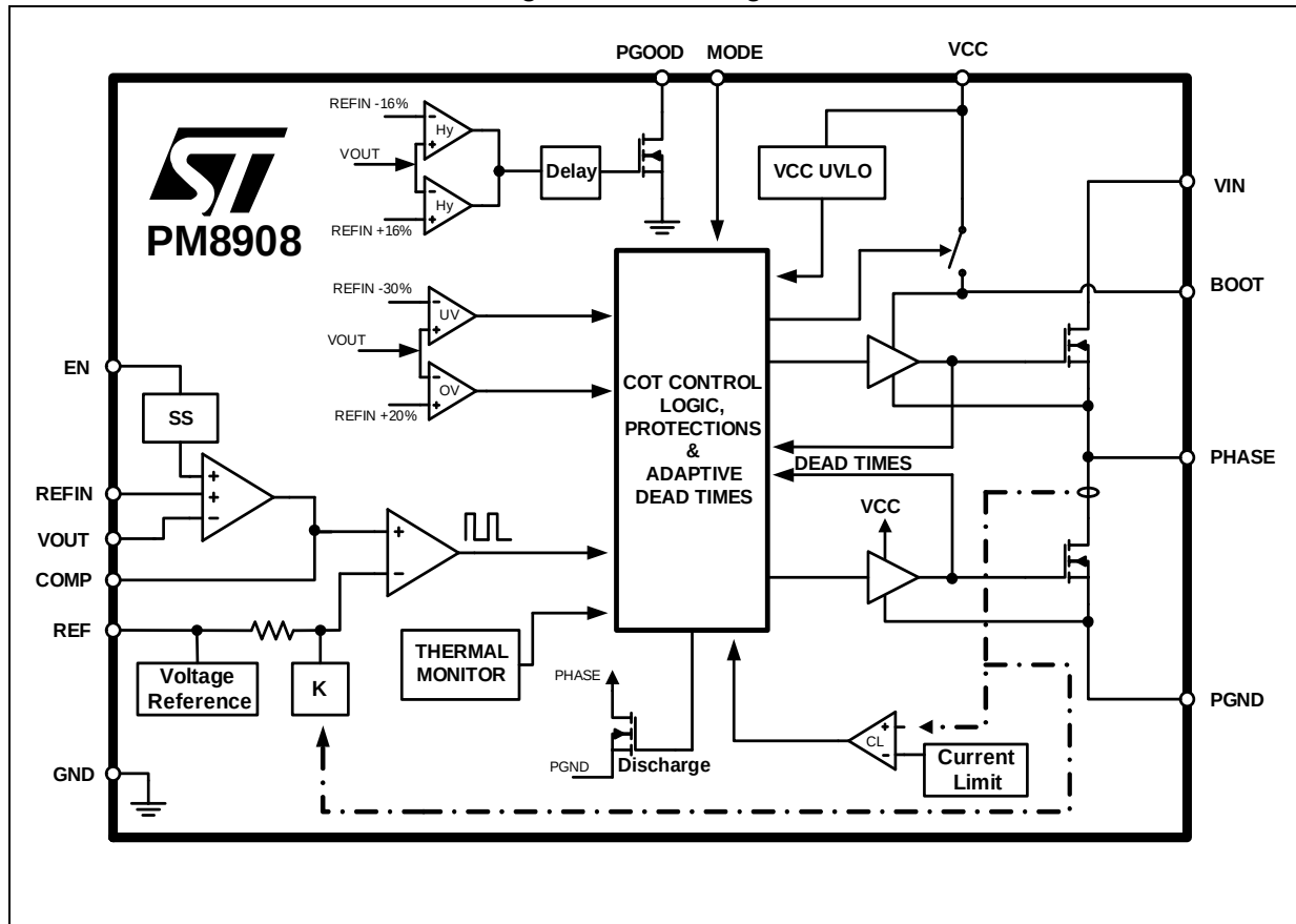
Figure 3. Block diagram
