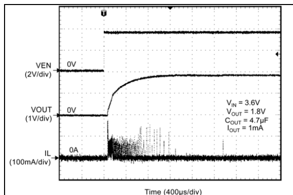
FIGURE 2-19: Start-Up, ( I_{OUT} = 1 \text{ mA} ).
