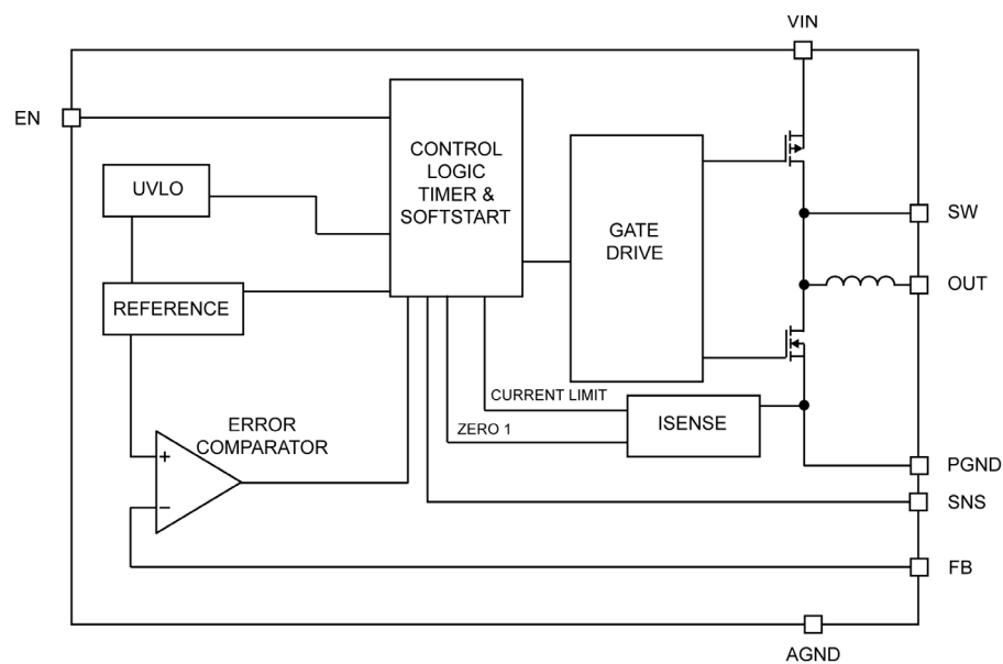
Simplified MIC33050 Adjustable Functional Block Diagram
