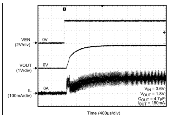
FIGURE 2-21: Start-Up, ( I_{OUT} = 150 \text{ mA} ).
