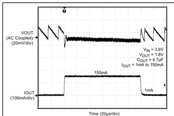
FIGURE 2-20: Load Transient, (1 mA to 150 mA).
