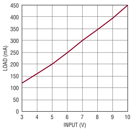
Figure 4. DC2186A-A Maximum Load Current vs Input Voltage
