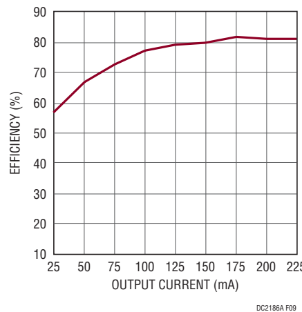
Figure 9. DC2186A-B Efficiency at 12V IN
