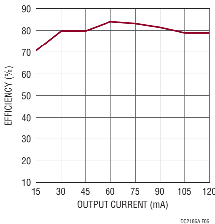
Figure 6. DC2186A-A Efficiency at 3V IN
