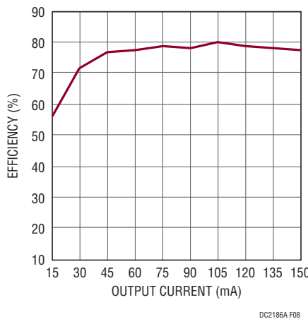
Figure 8. DC2186A-B Efficiency at 5V IN
