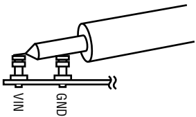
Figure 3. Measuring Input or Output Ripple
