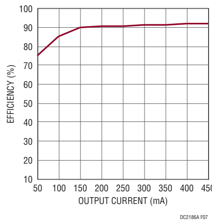
Figure 7. DC2186A-A Efficiency at 10V IN
