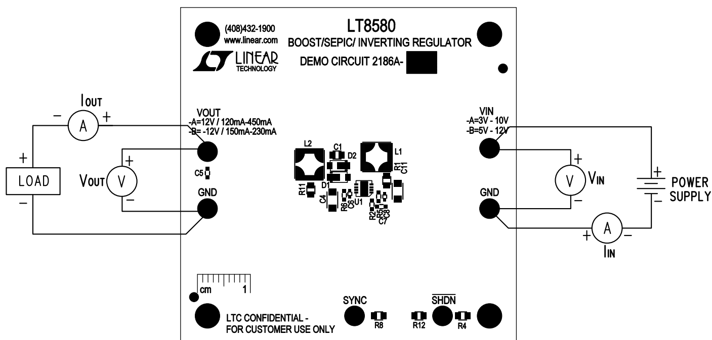
Figure 1. DC2186A-A Proper Equipment Setup
