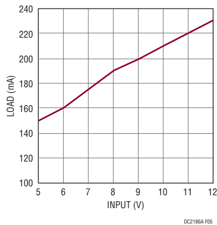
Figure 5. DC2186A-B Maximum Load Current vs Input Voltage
