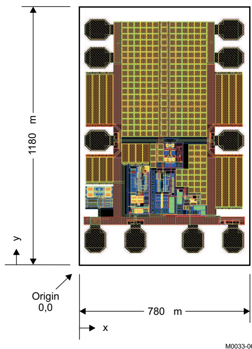
Figure 17. Chip Layout
