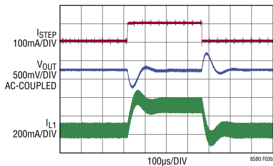
(3b) Transient Response Is Better
