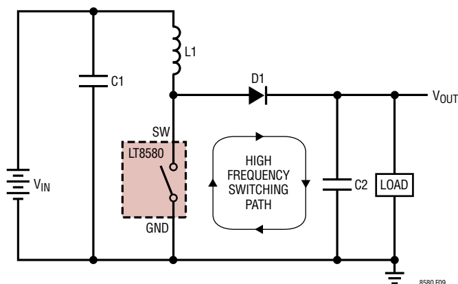
Figure 9. High Speed "Chopped" Switching Path for Boost Topology
