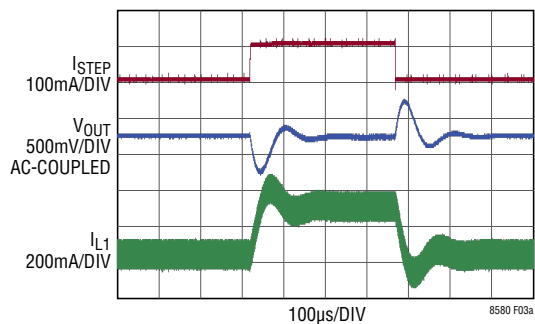
(3a) Transient Response Shows Excessive Ringing
