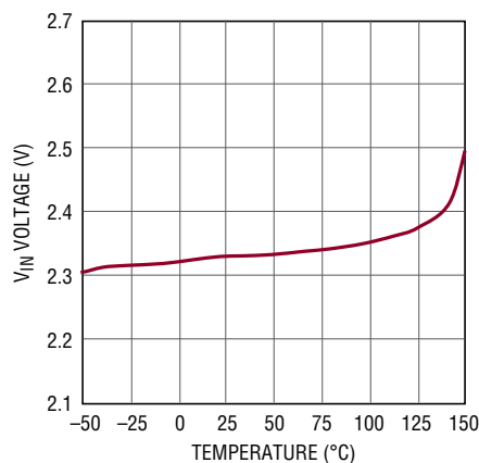
Internal UVLO
