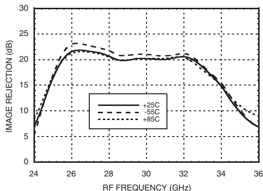
Image Rejection vs. Temperature @ LO= +2 dBm, Vdd= +4V
