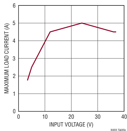
Maximum Load Current vs V_{IN} . BIAS Tied to LTM8003 GND
