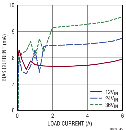
BIAS Current vs Load Current V_{OUT} = 8\text{V} , BIAS = 5V
