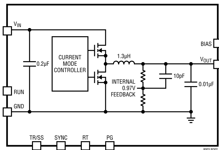
LTM8003-3.3 Block Diagram
