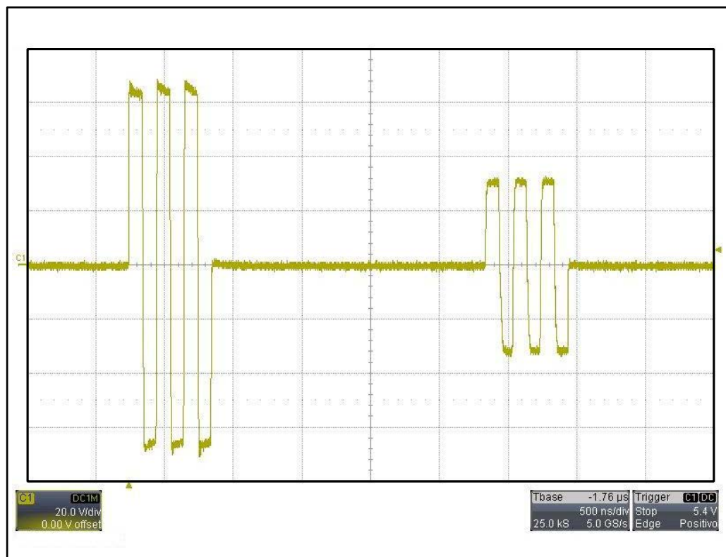
Figure 2: XDRC output in DUPLEX mode from single channel - PW and CW composition example
