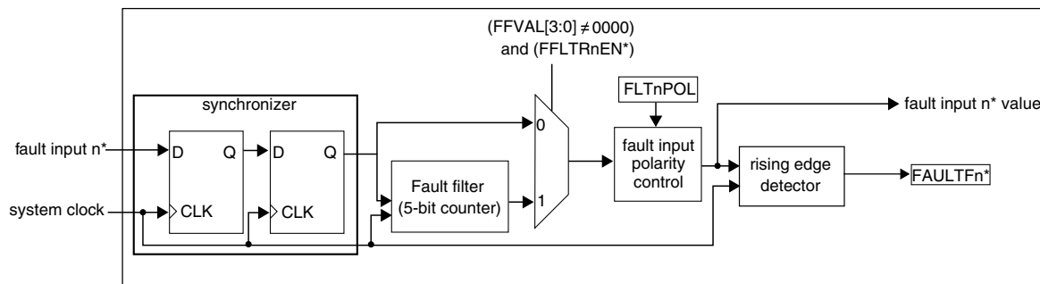
Figure 38-233. Fault input n control block diagram
