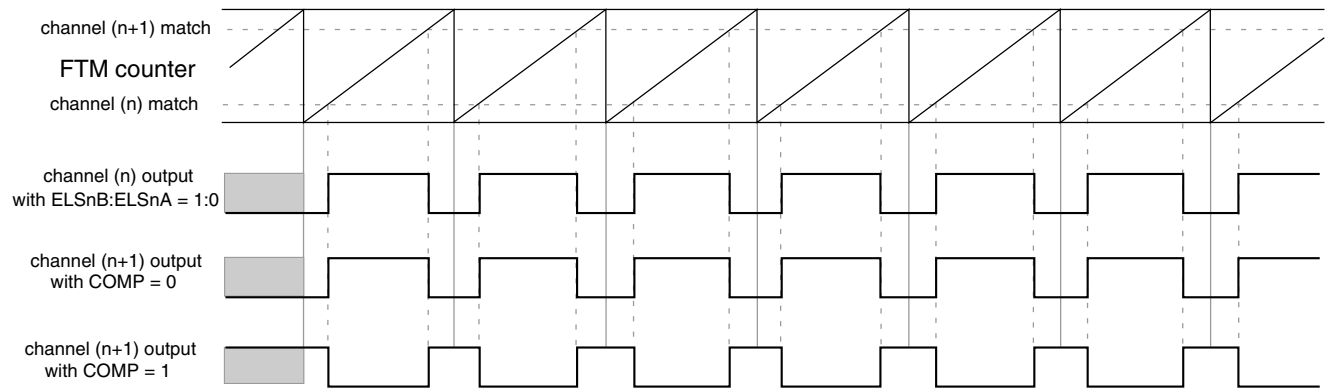
Figure 38-203. Channel (n+1) output in Complementary mode with (ELSnB:ELSnA = 1:0)
