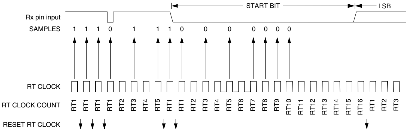
Figure 48-160. Start bit search example 1 ( C7816[ISO\_7816E] = 0 )
