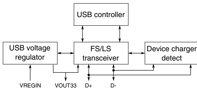
Figure 3-44. USB Subsystem Overview
