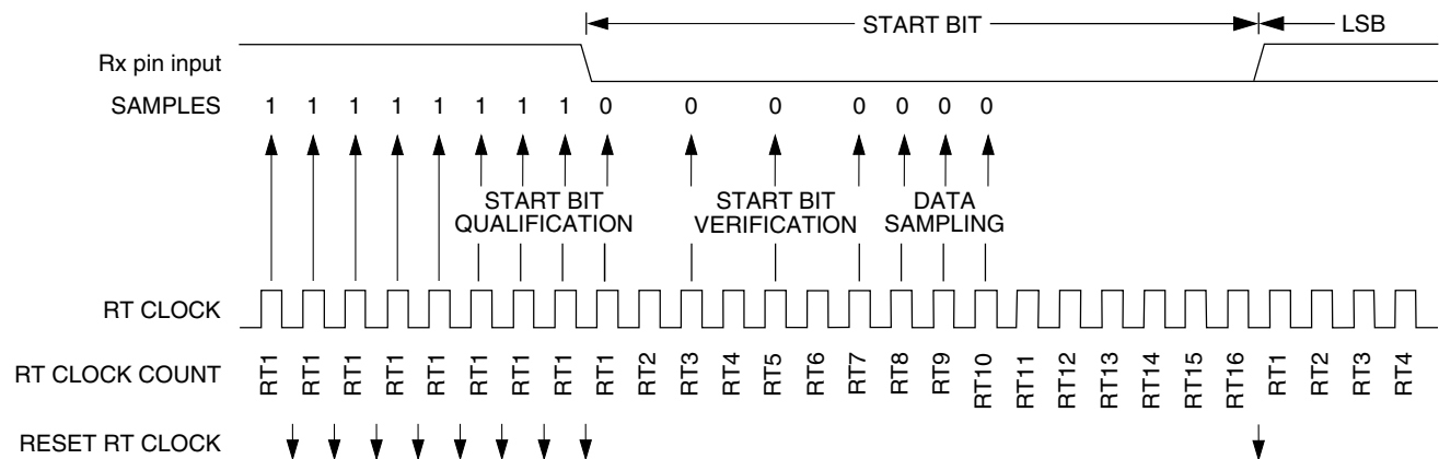
Figure 48-159. Receiver data sampling
