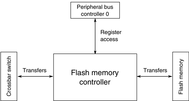
Figure 3-22. Flash memory controller configuration
