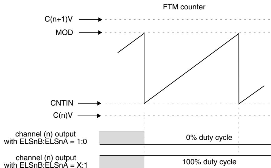
Figure 38-193. Channel (n) output if C(n)V and C(n+1)V are not between CNTIN and MOD
