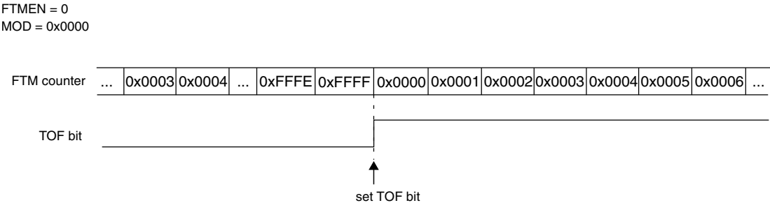
Figure 38-172. Example when the FTM counter is free running
