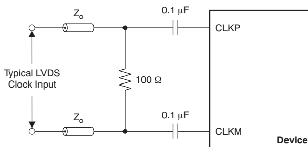
Figure 79. LVDS Clock Driving Circuit
