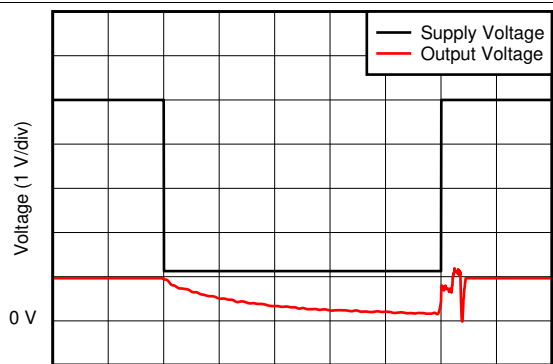
Figure 25. Noninverting Differential Input Overload
