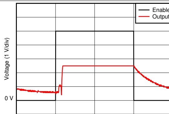
Figure 26. Start-Up Response
