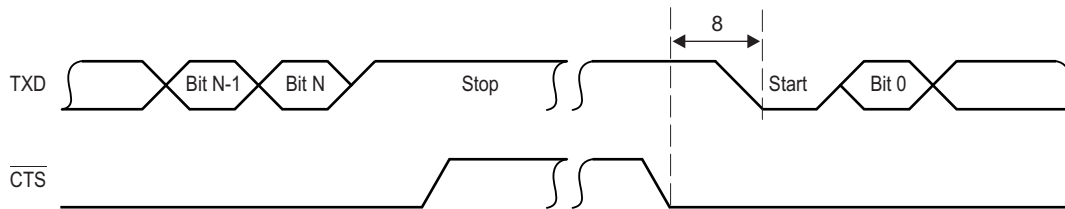
Figure 10-39. UART CTS (Clear-to-Send Input) — Autoflow Timing Waveform
