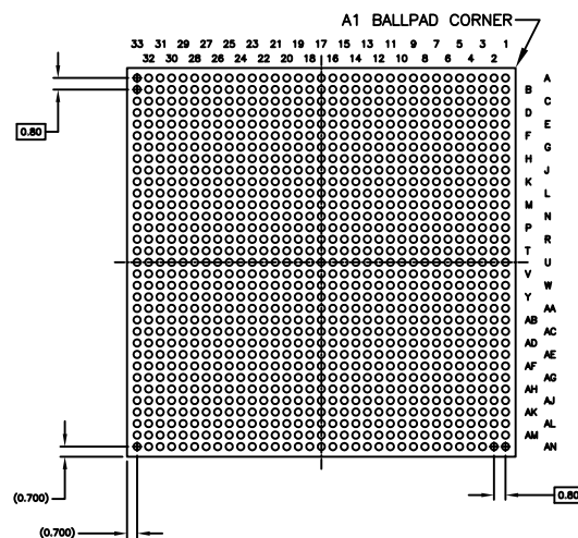
BOTTOM VIEW 1089 SOLDER BALLS
