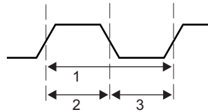
Figure 10-35. HyperLink Station Management Clock Timing
