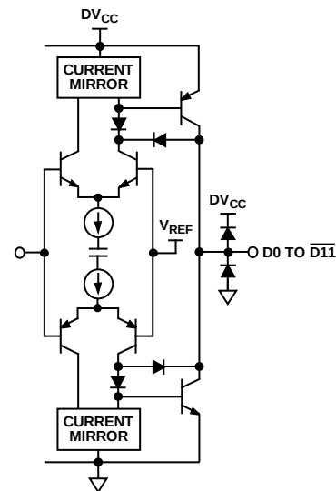
Figure 23. Digital Output Stage
