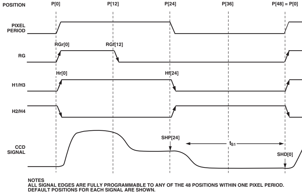
Figure 7. High Speed Timing Default Locations
