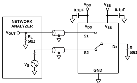
Figure 29. Channel-to-Channel Crosstalk
