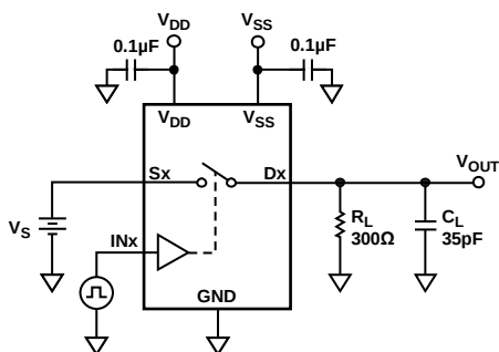
Figure 30. Switching Times, t_{ON} and t_{OFF}
