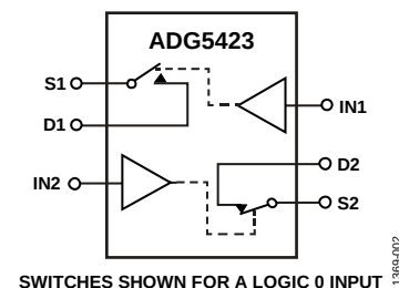
Figure 2. ADG5423
