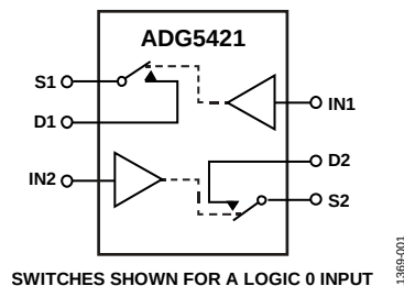
Figure 1. ADG5421
