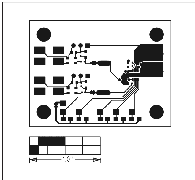
Figure 3. MAX8630X EV Kit PCB Layout—Component Side
