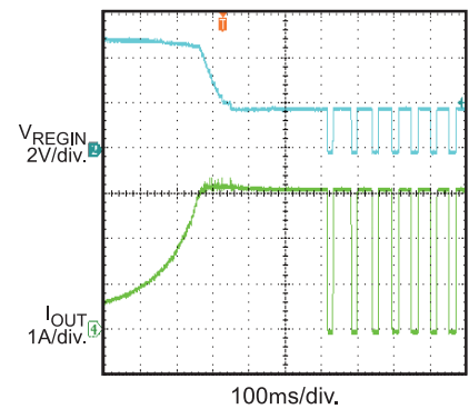
Input Current Limit R_{LIMIT} = 1.2k
