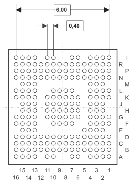
Figure 3. TPS65950 Mechanical Package -- Top View
