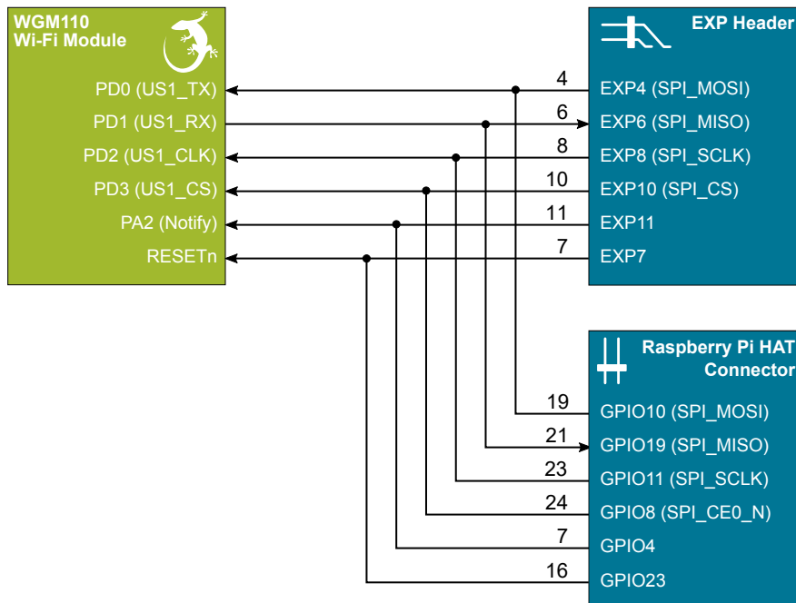
Figure 3.3. SPI Peripheral Routing on the WGM110 Wi-Fi Expansion Kit
