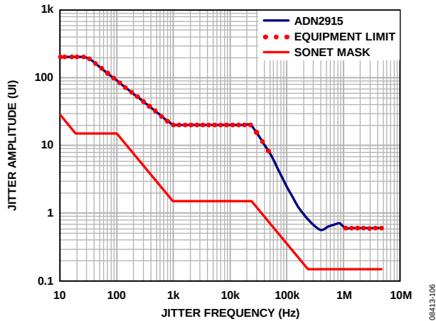
Figure 12. Jitter Tolerance: OC-12
