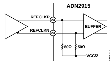
Figure 30. DC-Coupled, Differential REFCLKx Configuration
