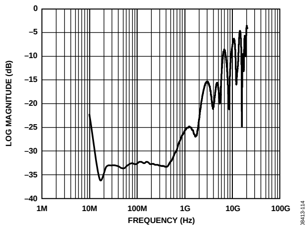
Figure 14. Typical S11 Spectrum Performance
