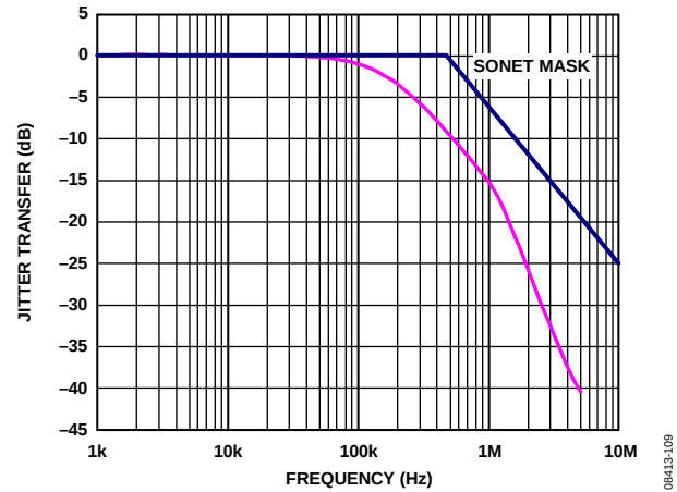
Figure 15. Jitter Transfer: OC-12
