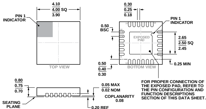
Figure 41. 24-Lead Lead Frame Chip Scale Package [LFCSP] 4 mm × 4 mm Body and 0.75 mm Package Height (CP-24-7)
