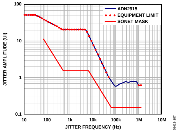
Figure 13. Jitter Tolerance: OC-3
