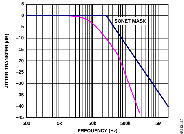
Figure 16. Jitter Transfer: OC-3
