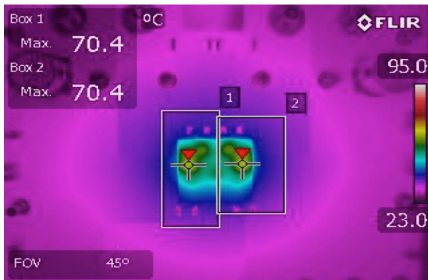
Figure 7. Thermal Capture at 12V_{IN} , 1.2V_{OUT1} at 10A and 1V_{OUT2} at 10A ( T_A = 25^{\circ}C , 200LFM Airflow and No Heat Sink)
