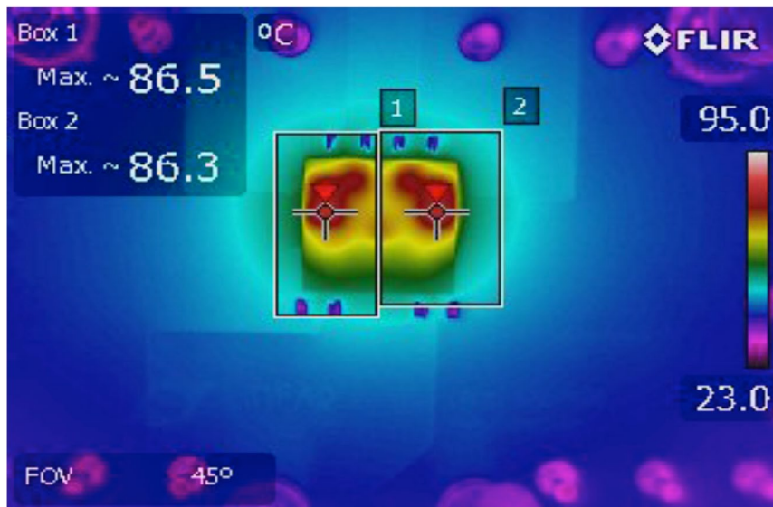
Figure 6. Thermal Capture at 12V_{IN} , 1.2V_{OUT1} at 10A and 1V_{OUT2} at 10A ( T_A = 25^{\circ}C , No Forced Airflow and No Heat Sink)
