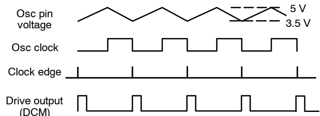
Figure 37. Oscillator Mode Timing Diagram in DCM
