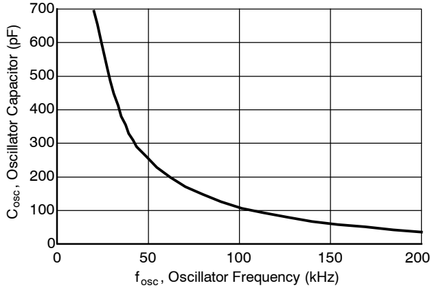
Figure 38. Osc Pin Frequency Setting
