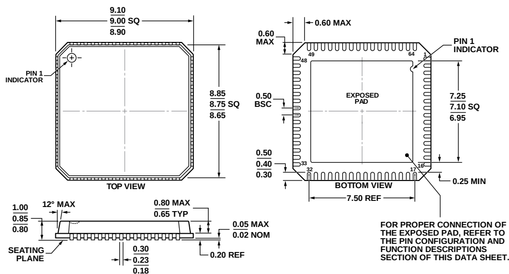
Figure 10. 64-Lead Lead Frame Chip Scale Package [LFCSP_VQ] 9 mm x 9 mm Body, Very Thin Quad (CP-64-3) Dimensions shown in millimeters
