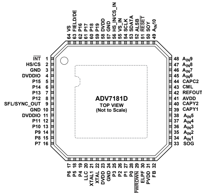
Figure 6. Pin Configuration
