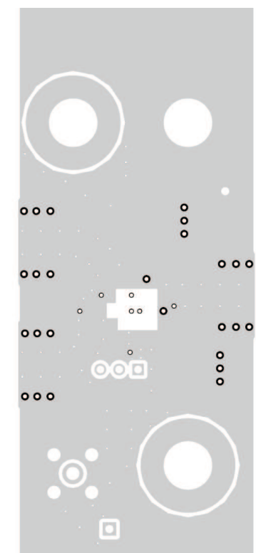
Figure 3. Ground Layer 2
