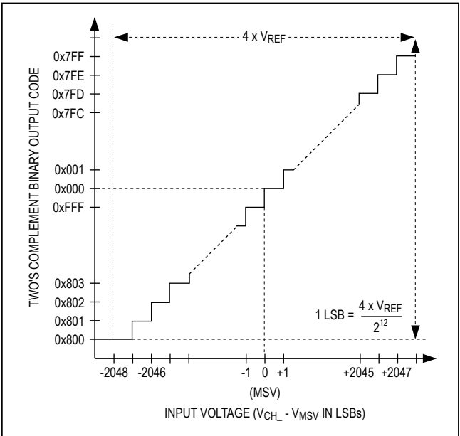
Figure 13. ±5V Bipolar Transfer Function
