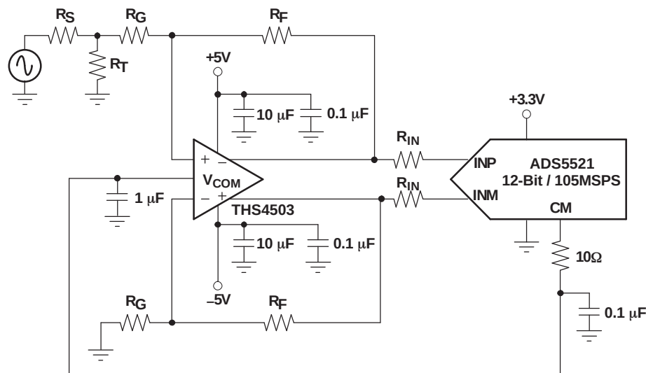
Figure 42. Using the TMS4503 with the ADS5521
