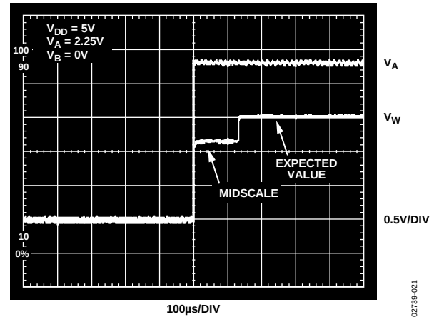
Figure 21. Power-On Reset, V_A = 2.25\text{ V} , V_B = 0\text{ V} , Code = 1010101010 B
