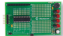
PICKit Low Pin Count Development Board (DM164130-9)
