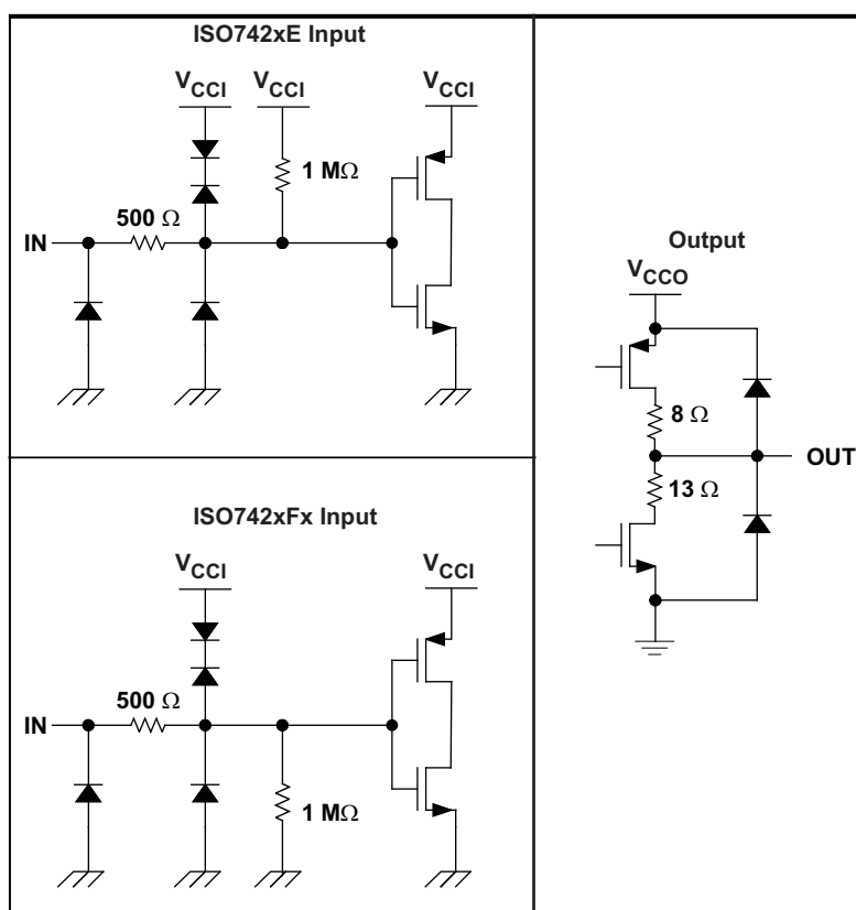
Figure 22. Device I/O Schematics
