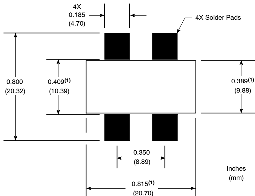
Figure 18. PCB Pad Layout for OM-780-4L
