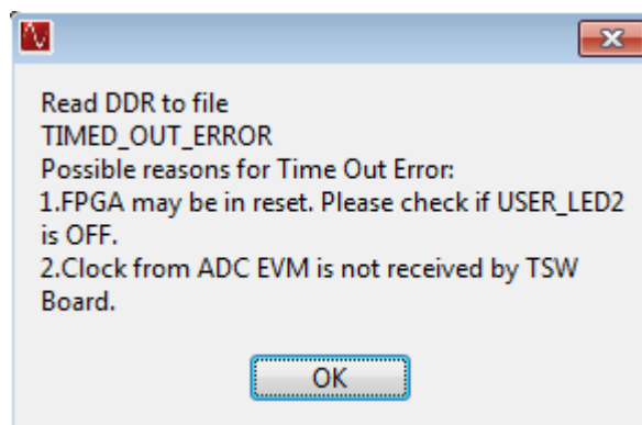
Figure 69. Read DDR Error for No Capture
