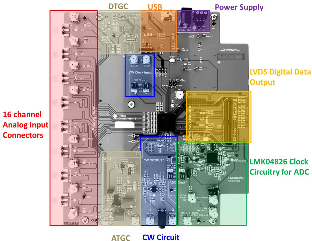
Figure 55. AFE5818 EVM Circuits Map
