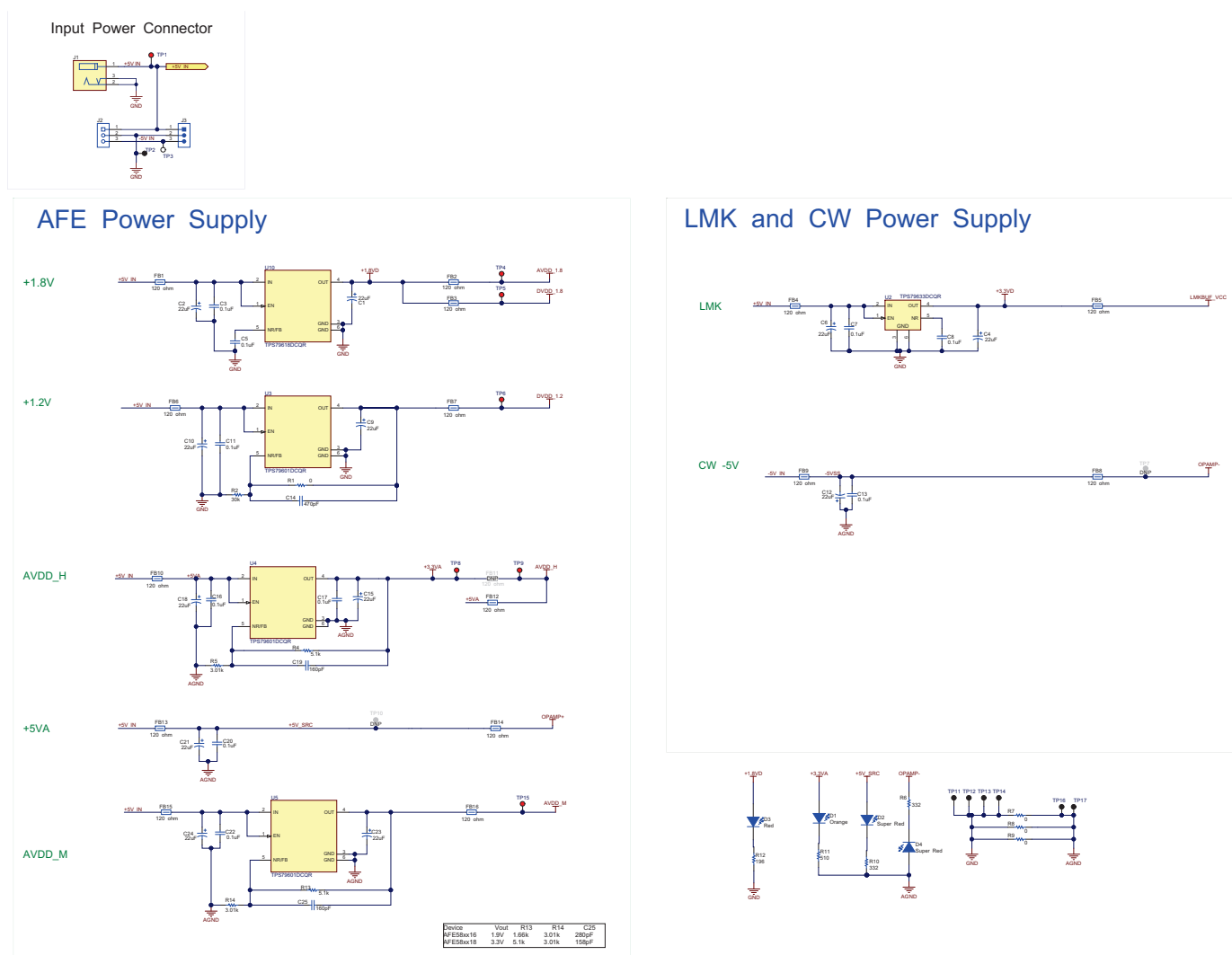
Figure 57. AFE5816 Rev C EVM Schematic 1 of 11
