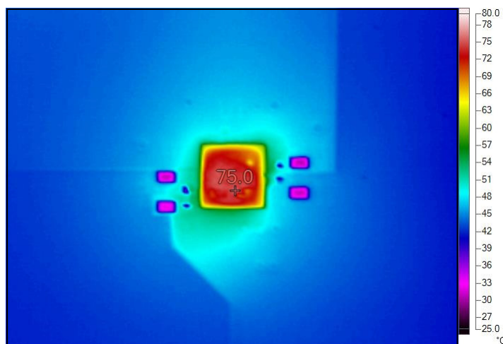
Figure 4. Measured Thermal Capture at 12V IN and 1.5V OUT , 12A OUT at 25°C Ambient with No Airflow
