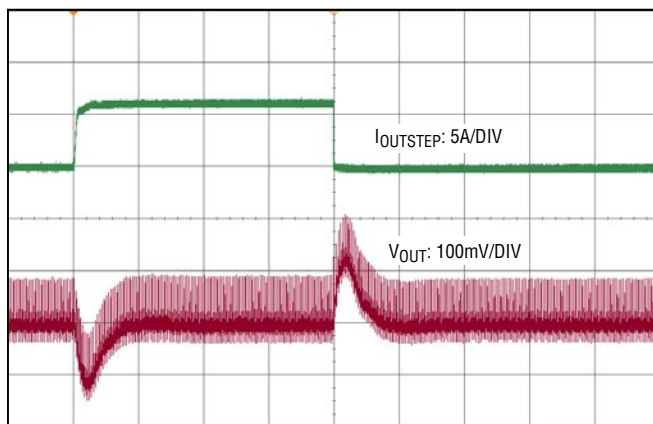
Figure 3. Load Transient (6A to 12A) Response Waveform at 12V IN and 1.5V OUT , 50µs/DIV
