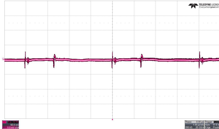
Figure 7: 3.3V/25W Flyback Output Voltage Ripple at Full Load measured with 20 MHz bandwidth
