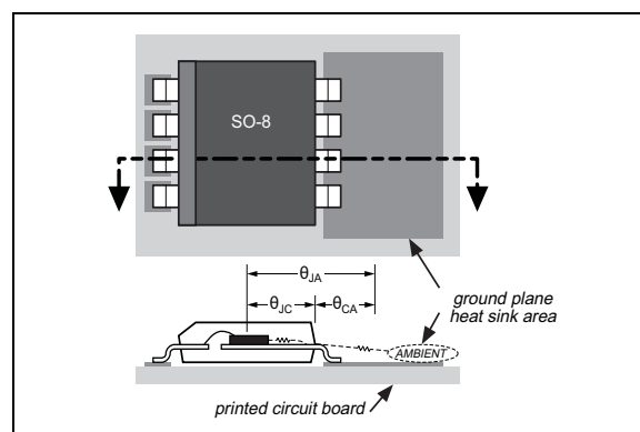
FIGURE 4-1: Thermal Resistance.
