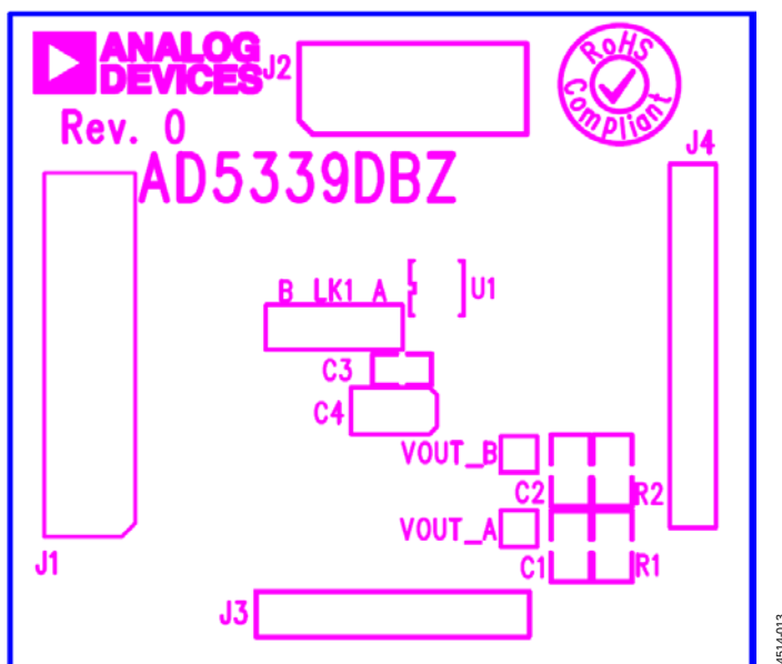
Figure 14. EVAL-AD5339DBZ Daughter Board Component Placement
