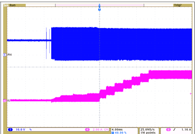
Figure 21. Battery Charging Soft-Start
