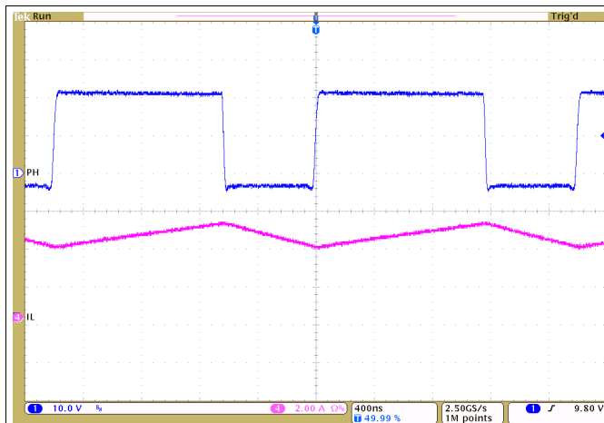
Figure 20. Continuous-Conduction Mode Switching Waveform
